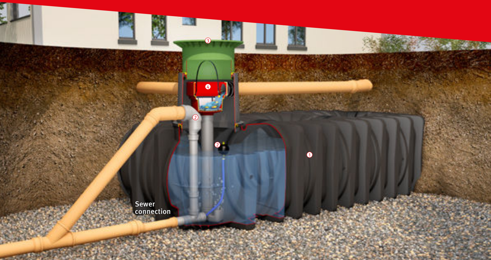
Platin XL/XXL detention cistern Including detention set
